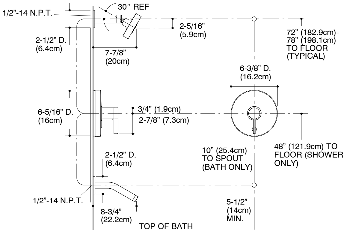
PRODUCT DIAGRAM
